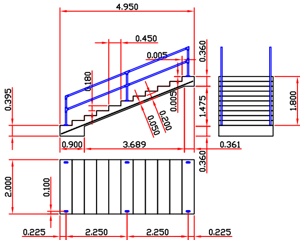
CONCRETE STAIR DETAIL
